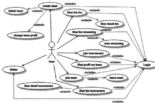
Gambar 2. Usecase Diagram User
