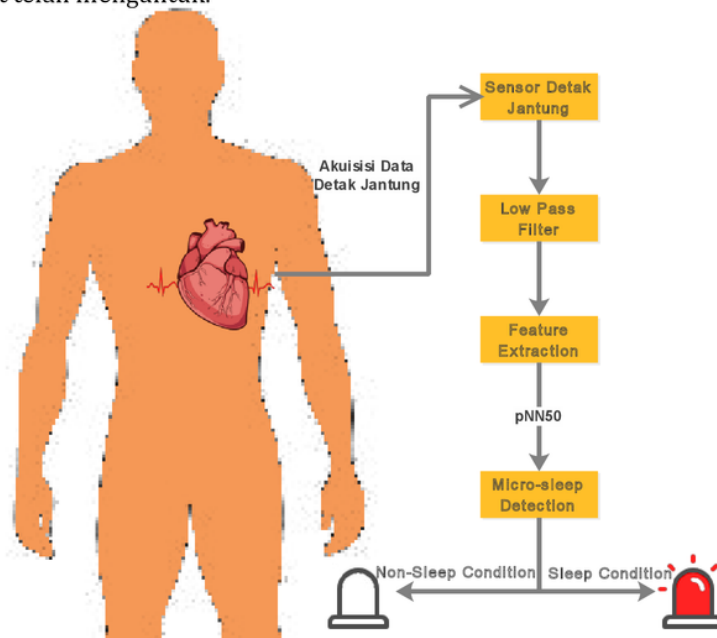
Gambar 4. Blok Diagram Deteksi Micro-sleep
