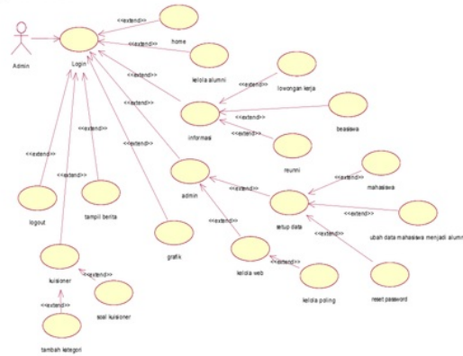
Gambar 2.1 Use Case Diagram Admin
