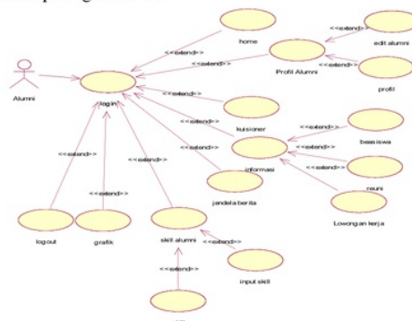
Gambar 2.2 Use case Diagram Alumni
