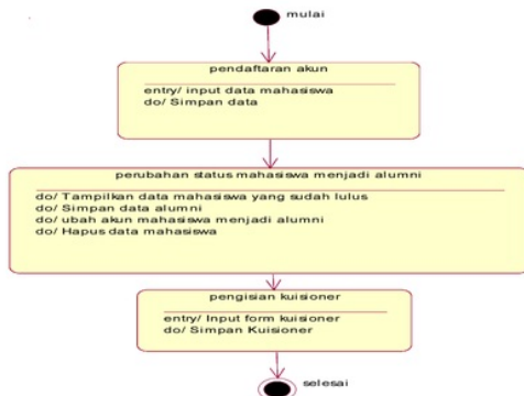
Gambar 2.12: Statechart Diagram Tracer Study Teknik Informatika Universitas Muria Kudus
