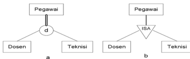
Gambar 3. Notasi generalization dan specialization
