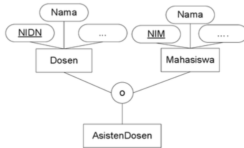
Gambar 11. Pewarisan ganda ( multiple inheritance )
