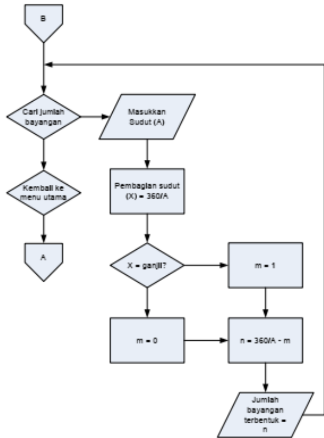
Gambar 2. Flowchart Menu Cermin Datar
