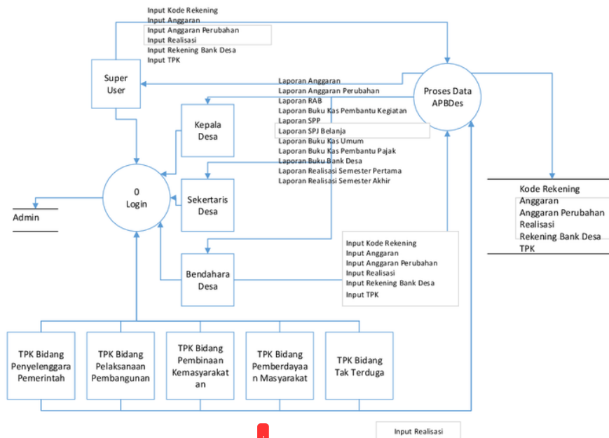
Gambar 2. DFD level 0
