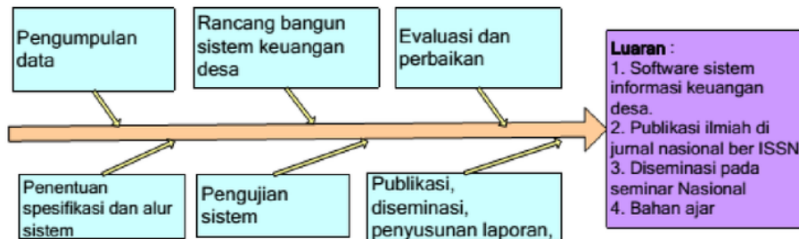
Gambar 1. Diagram Fishbone
