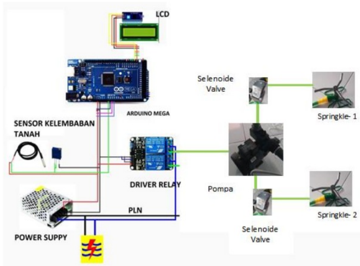
Gambar 2. Wiring system
