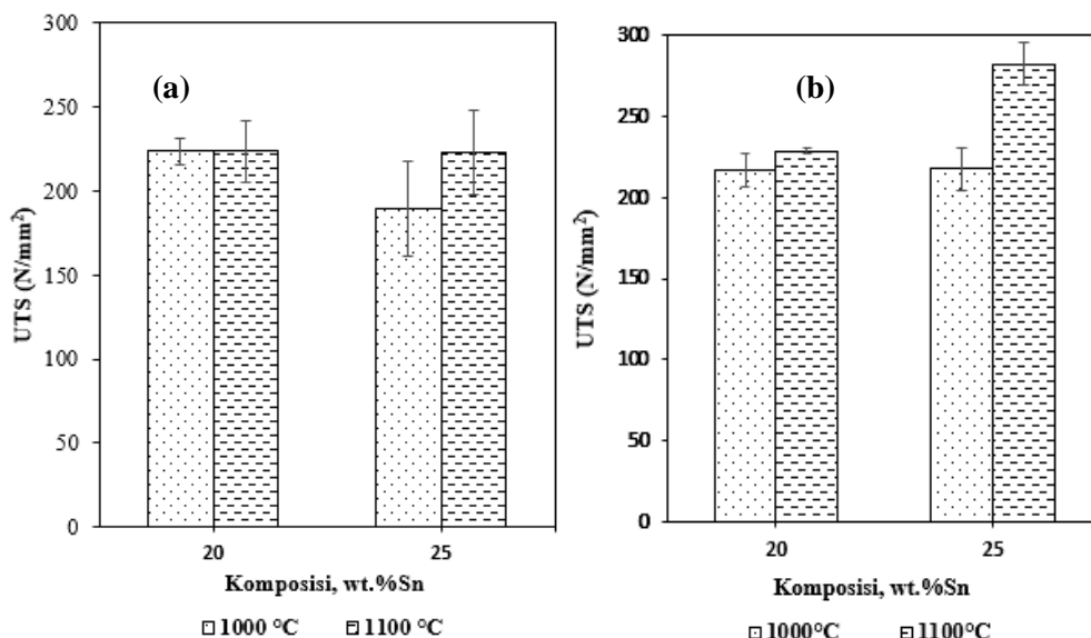
Gambar 8. Kekuatan tarik paduan perunggu timah (a) Sand casting/SC (b) Investment casting/IC
