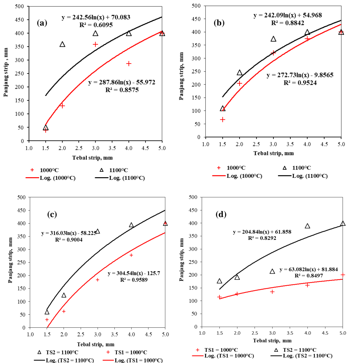
Gambar 5. Panjang fluiditas (a) 20wt.%Sn/SC; (b) 20wt.%Sn/IC; (c) 25wt.%Sn/SC; (d) 25wt.%Sn/IC
