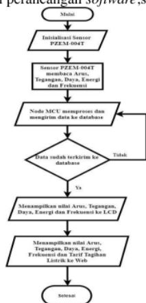
Gambar 5. Diagram Alur Perancangan Software
