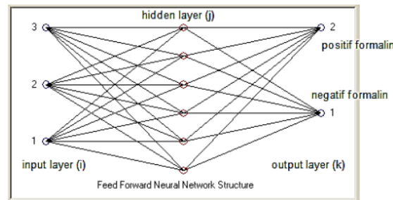
Figure 4. Three-Layer Multi-Layer Perceptron Scheme
