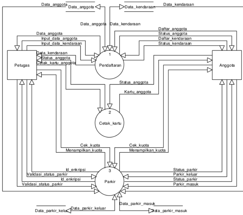
Gambar 5. DFD Level 0
