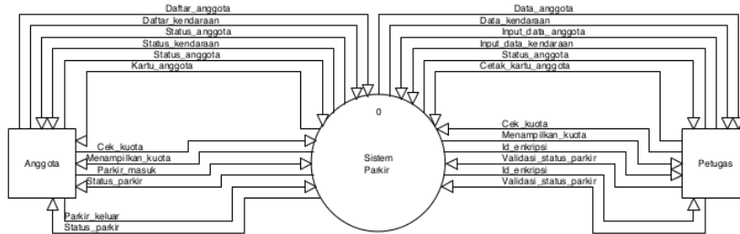
Gambar 4. Context Diagram
