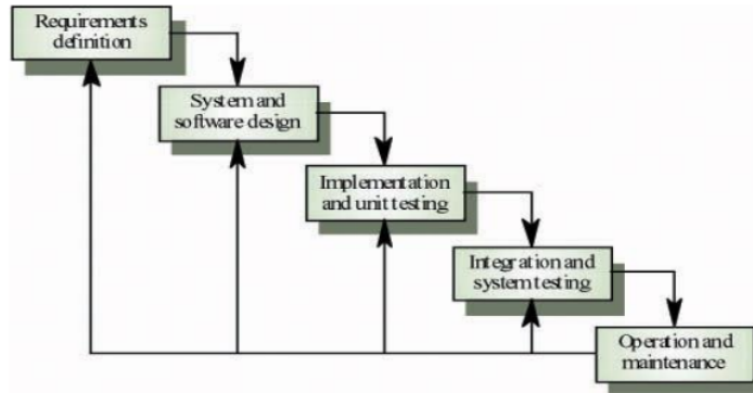
Gambar 2. Waterfall Model [9]
