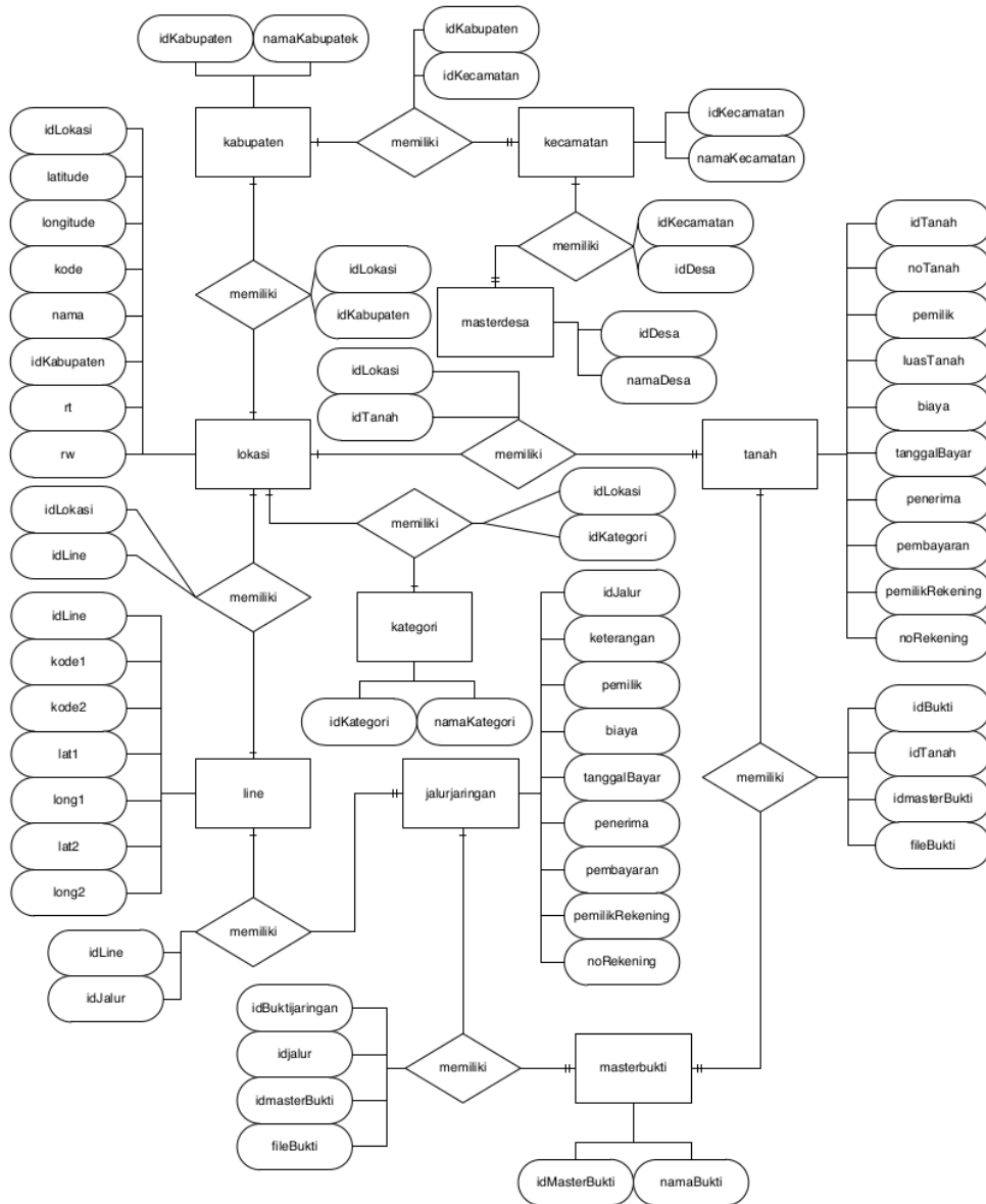
Gambar 7 ERD (Entity Relationship Diagram)
