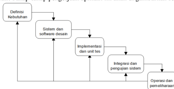
Gambar 1. Metodologi Waterfall
