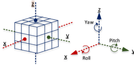
Figure 2. Cube and its rotation
