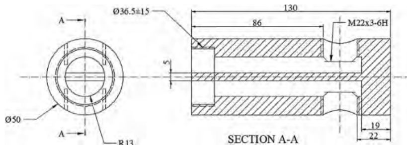
Fig. 2. The configuration of the simple T mixer.
