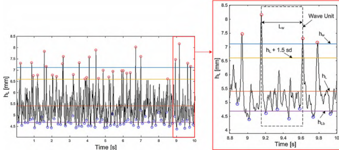
Fig. 9. The example of local film thickness ( J_L = 0.03 m/s and J_G = 13 m/s).
