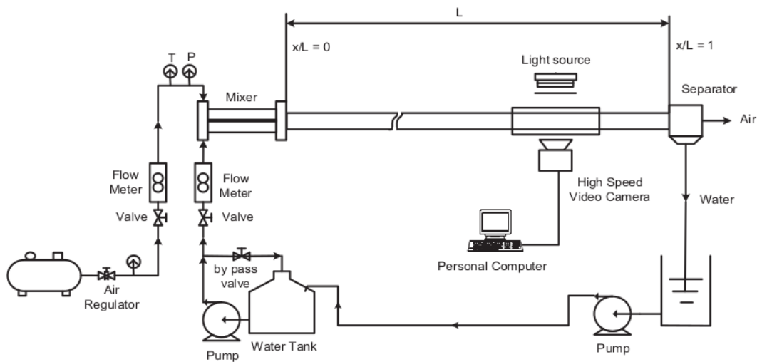
Fig. 1. The schematic diagram of the experimental apparatus.
