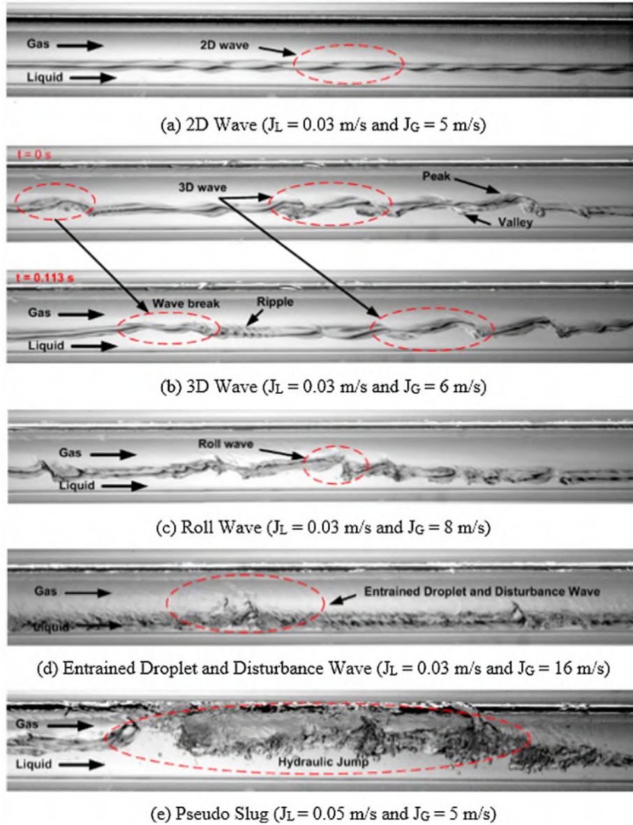
Fig. 10. The example of various wave types.
