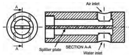
Fig. 2. Configuration of air-water mixer.
