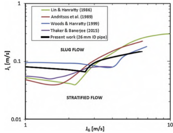
Fig. 17. Transition line from stratified to slug flows.
