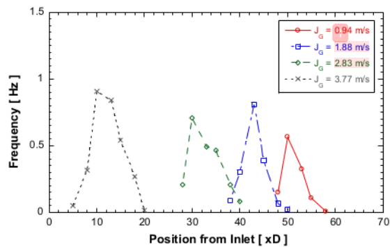
Fig. 27. The distribution of slug initiation position ( J_L = 0.31 m/s).
