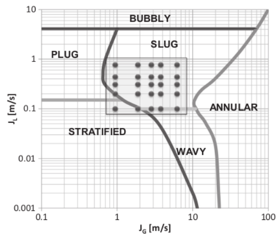
Fig. 3. Experimental data plotted on the Mandhane et al. [15] map.
