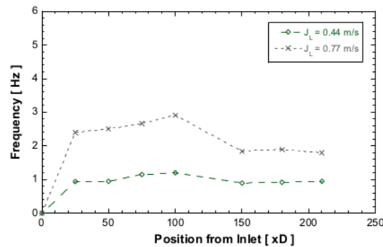
Fig. 32. The effects of J_L to the evolution of passing slug frequency along the pipe ( J_C = 6.2 m/s).
