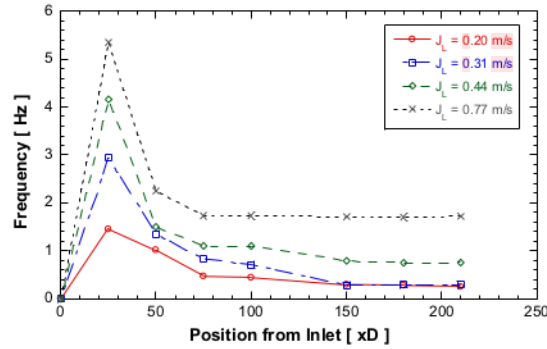
Fig. 31. The effects of J_L to the evolution of passing slug frequency along the pipe ( J_C = 3.77 m/s).
