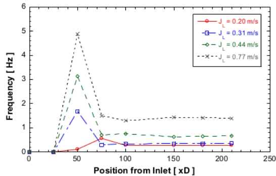
Fig. 30. The effects of J_L to the evolution of passing slug frequency along the pipe ( J_C = 1.88 m/s).
