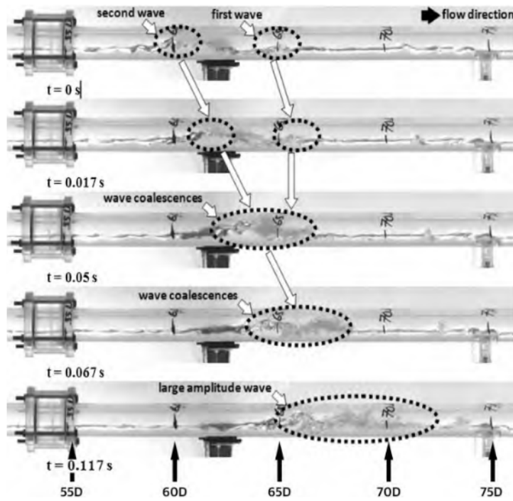
Fig. 5. Snapshot of the interfacial behavior of the roll waves coalescence mechanism at initiation section 55 D–75 D ( J_L = 0.10 m/s and J_G = 6.20 m/s).
