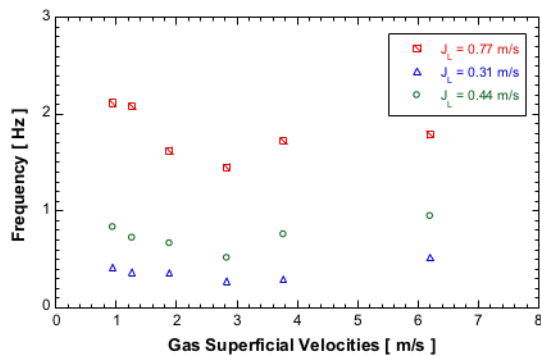
Fig. 33. Slug frequency at 210 D.
