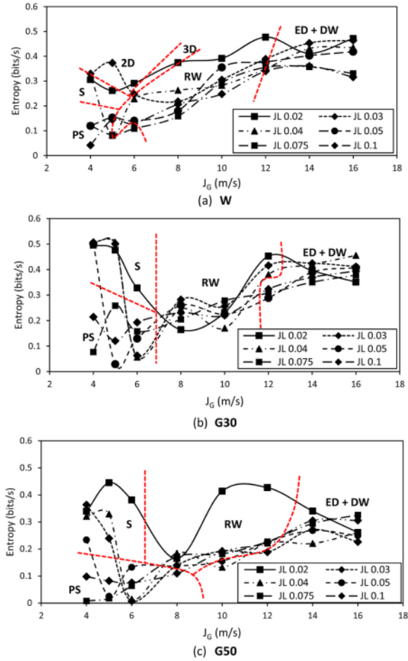
Fig. 12. The effect of the both J_L and J_G on the entropy of the fluctuations of the pressure gradient.
