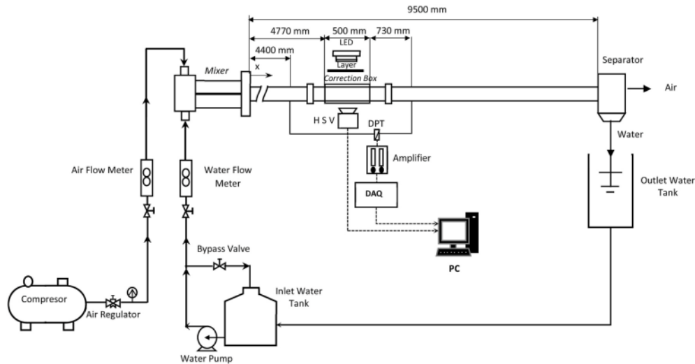
Fig. 1. Experimental apparatus.
