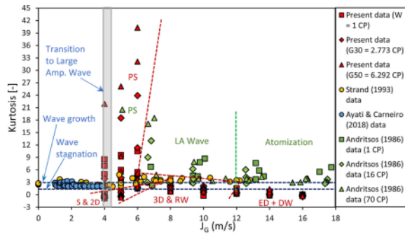
Fig. 11. The effect of J_G on the kurtosis.
