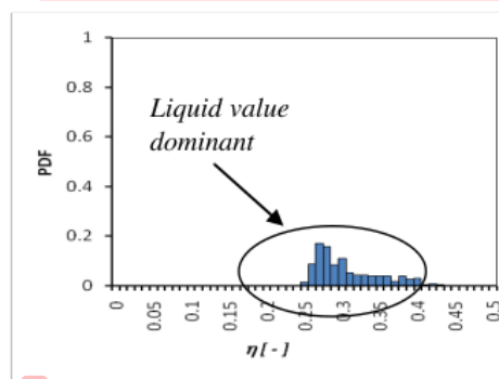
Gambar 7. Contoh PDF Aliran Stratified Wavy + Ripple ( J_L = 0,092 m/s dan J_G = 1,02 m/s)
