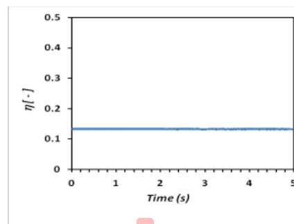
Gambar 3. Contoh Liquid hold-up Aliran Stratified Smooth ( J_L = 0,016 m/s dan J_G = 1,02 m/s)
