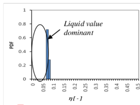
Gambar 4. Contoh PDF Aliran Stratified Smooth ( J_L = 0,016 m/s dan J_G = 1,02 m/s)
