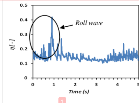
Gambar 9. Contoh Liquid Hold-Up Aliran Stratified Wavy + Roll ( J_L = 0,047 m/s dan J_G = 3.77 m/s)
