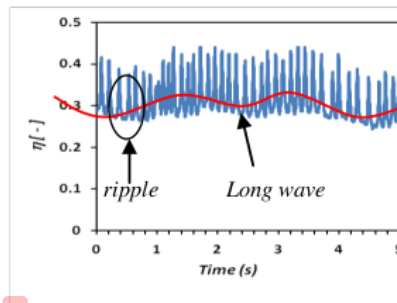
Gambar 6. Liquid Hold-Up Aliran Stratified Wavy + Ripple ( J_L = 0,092 m/s dan J_G = 1,02 m/s)
