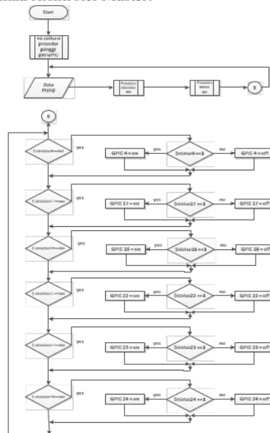
Gambar 3. Diagram Alir Program BASH Linux (raspbian pin) ke Box Relay
