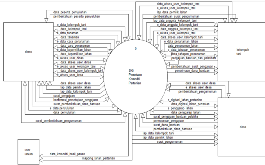
Gambar 8.2 DFD level 0
