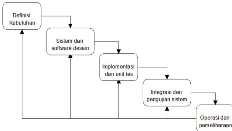
Gambar 7.1. Metodologi Waterfall
