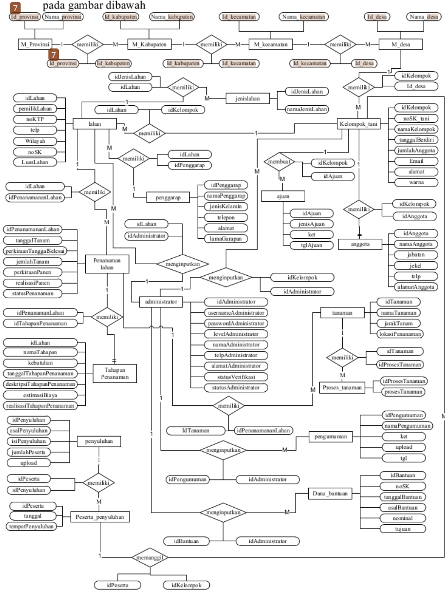
Gambar 8.3. Entity Relationship Diagram
